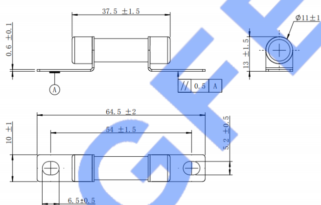
Surface Mount*1xxH-10R 表面安装连接
